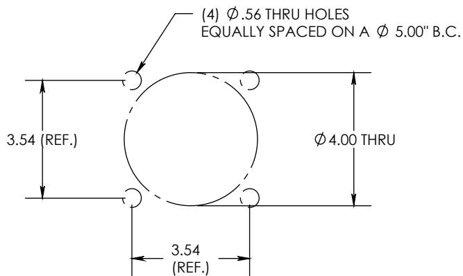
RECOMMENDED MOUNTING DETAIL
